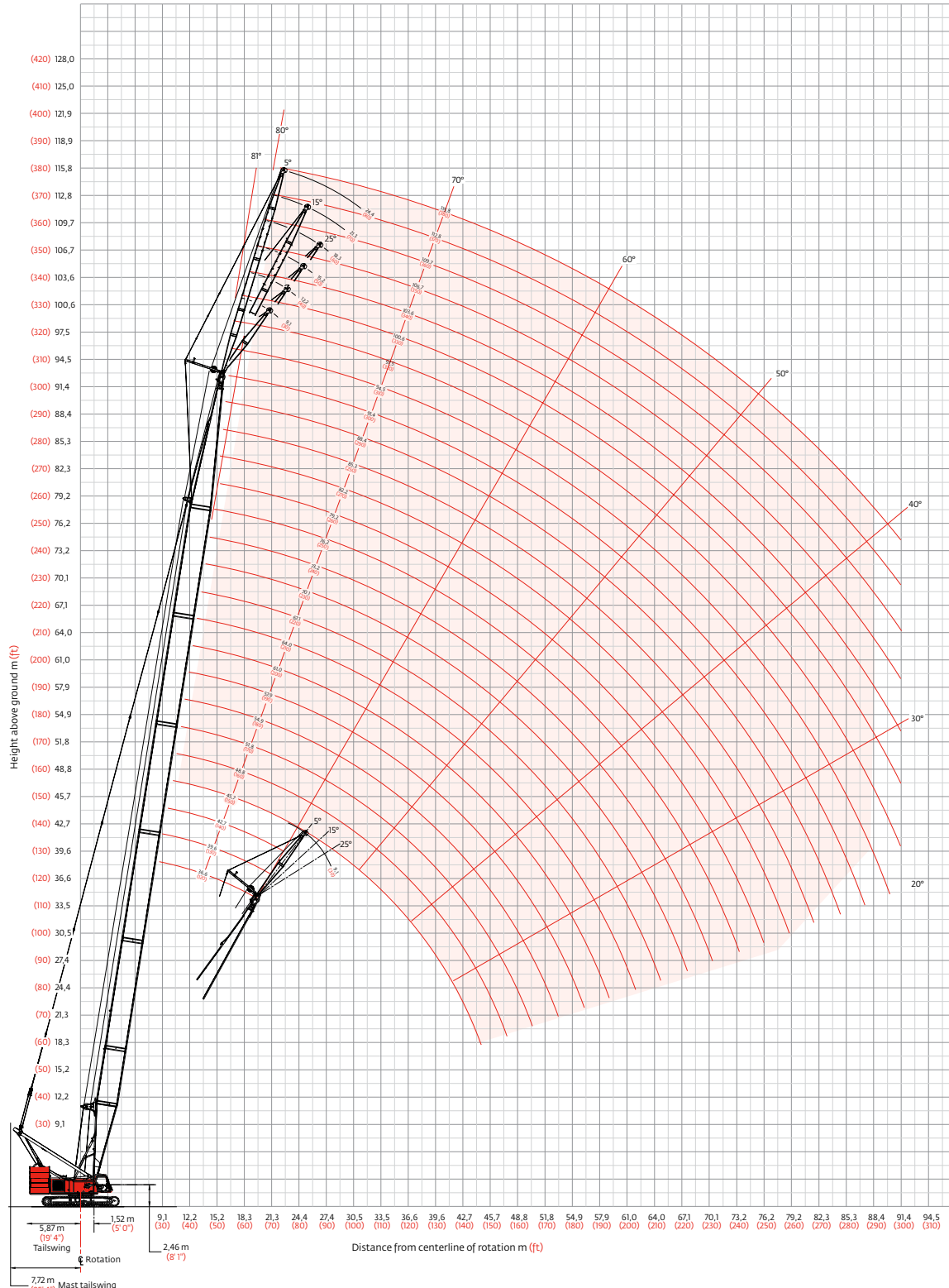
No. 134 Fixed Jib on No. 82LR Boom
